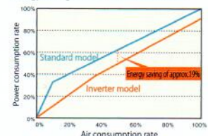
Energy-saving chart for the inverter model
