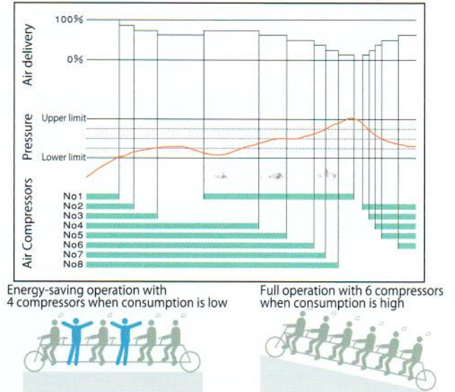
Operation of multi-stage control to achieve high energy-saving performance (multi-stage control)
