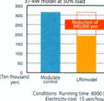
Consumption power saving by LRV (loaded and unloaded control) 37-kW model at 50% load
