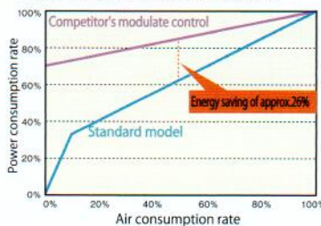
Energy-saving chart for the standard model
