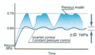
Constant pressure control for energy saving
